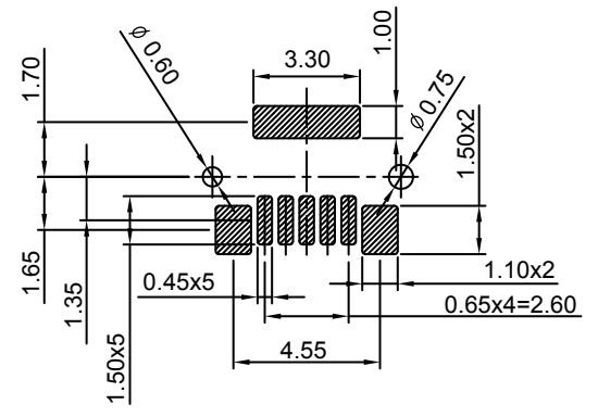
Recommended PCB Layout With Mounting Pegs
