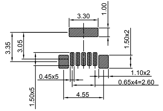
Recommended PCB Layout Without Mounting Pegs
