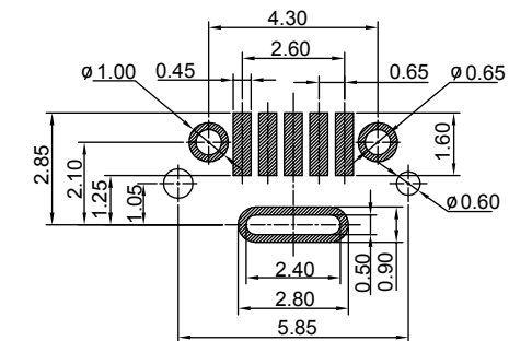
Recommended PCB Layout With Mounting Pegs
