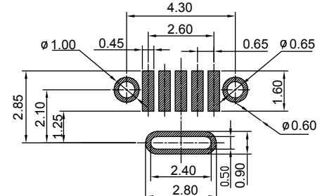
Recommended PCB Layout Without Mounting Pegs
