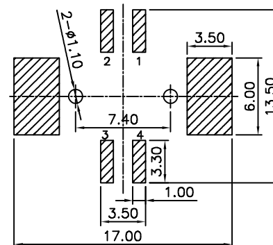
TOP VIEW RECOMMENDED PCB LAYOUT
