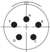
15-5/14-5 D5, 5 # 16, II
