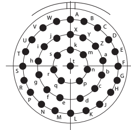
21-41/20-41 G41, 41 # 20, I
