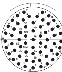
25-61/24-61 J61, 61 # 20, I
