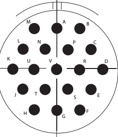
25-19/24-19 J19, 19 # 12, I
