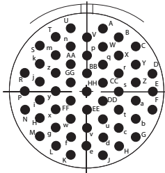
23-55/22-55 H55, 55 # 20, I
