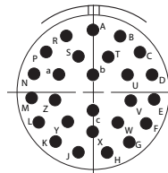
17-26/16-26 E26, 26 # 20, I
