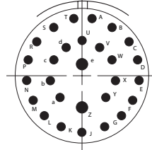
19-28/18-28 F28, 2 # 16, 26 # 20, I
