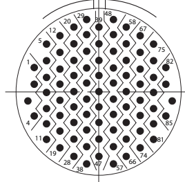
23-2*/22-2* 85 # 22, M
