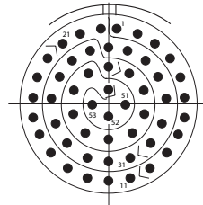
18-53* 53 # 22, M
