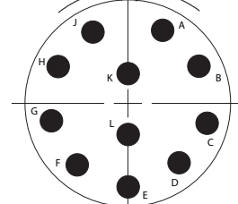
21-11 G11, 11 # 12, I
