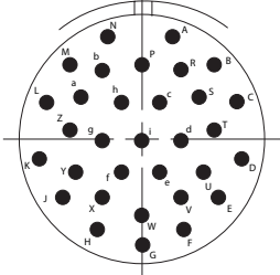
23-32/22-32 H32, 32 # 20, I
