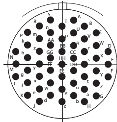
23-53/22-53 H53, 53 # 20, I
