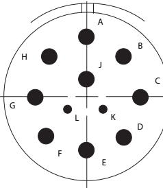
J11 9 # 10, 2 # 20, N
