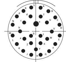
19-30/18-30 F30, 1 # 16, 29 # 20, I
