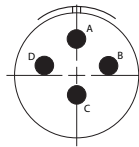
13-4/12-4 C4, 4 # 16, I
