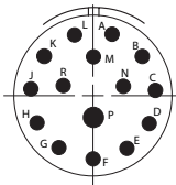
15-15/14-15 D15, 1 # 16, 14 # 20, I
