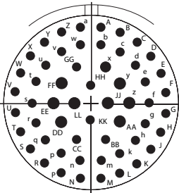
25-4/24-4 J4, 8 # 16, 48 # 20, I
