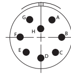
13-8/12-8 C8, 8 # 20, I
