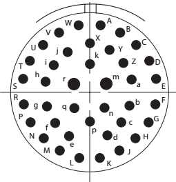
21-39/20-39 G39, 2 # 16, 37 # 20, I
