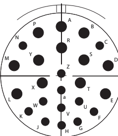
25-24/24-24 J24, 12 # 12, 12 # 16, I
