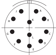
19-11/18-11 F11, 11 # 16, II
