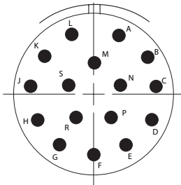
21-16/20-16 G16, 16 # 16, II
