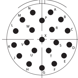
23-21/22-21 H21, 21 # 16, II
