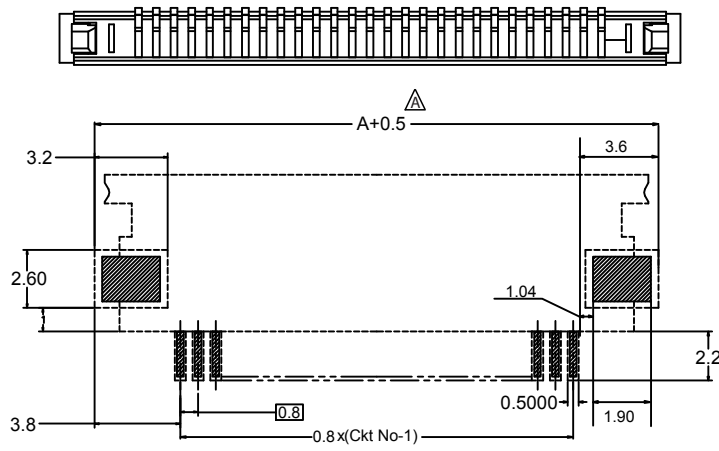
PCB LAYOUT
