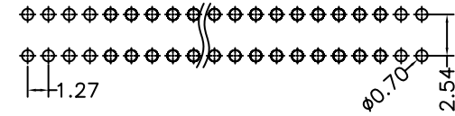
Recommended P.C.B Layout (Top Side)
