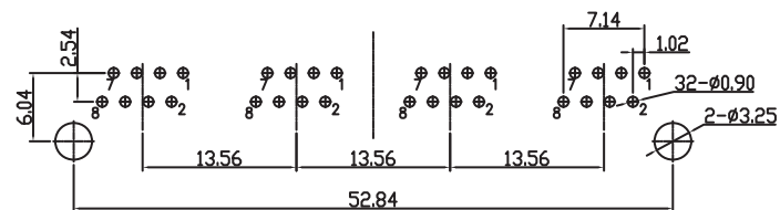
Recommended PCB Layout (Top View)
